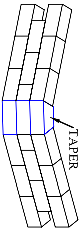
OUTSIDE ANGLE -NO BATTER (MSE WALL)
