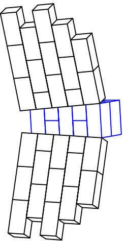
INSIDE ANGLE -WITH BATTER (MSE WALL)
