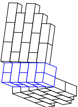
90° CORNER -WITH BATTER (MSE WALL)
