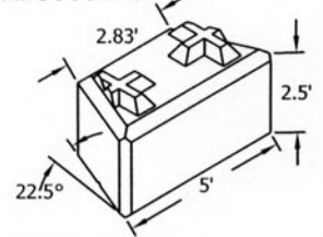
WEDGE APPROX. 3450LBS
