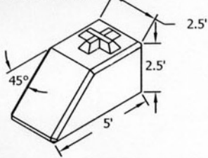
FLAT TOP TRANS. APPROX. 3450LBS
