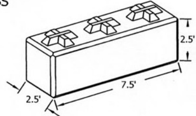
3-CROSS BEAM APPROX. 6480LBS
