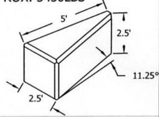
WEDGE APPROX. 3450LBS
