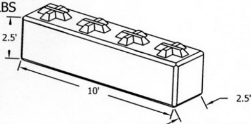
4-CROSS BEAM APPROX. 8640LBS
